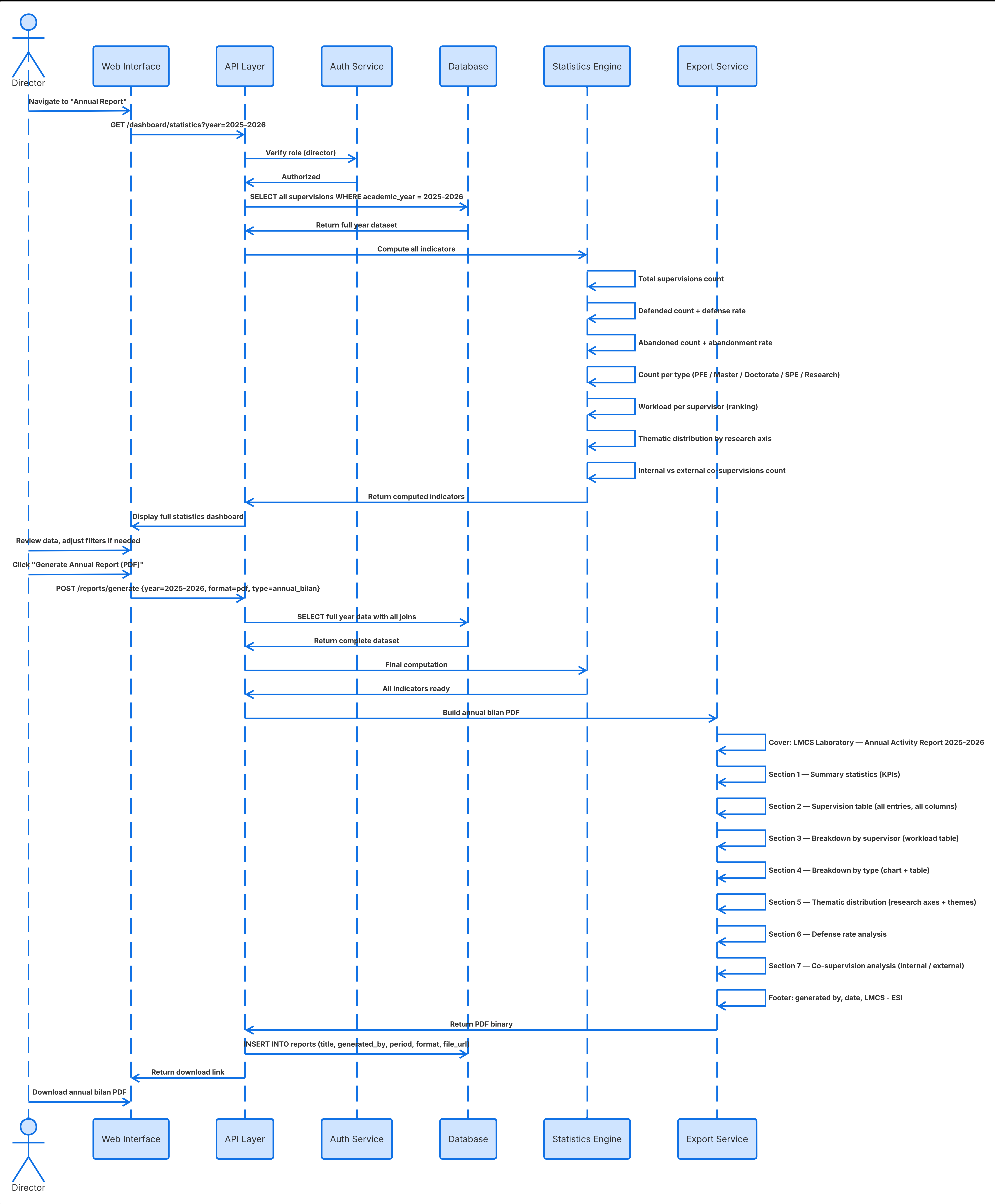
Annual Report Generation Flow
